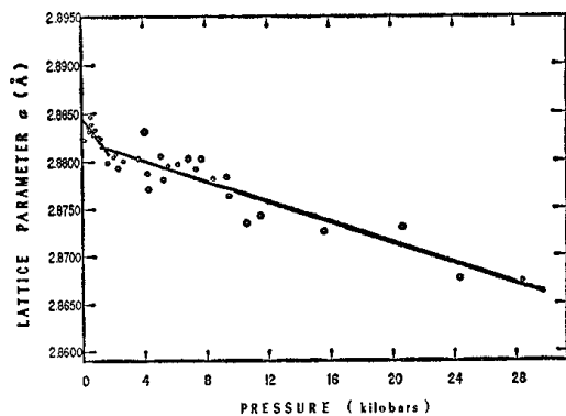
Fig. 1. Lattice parameters of chromium vs. pressure.
